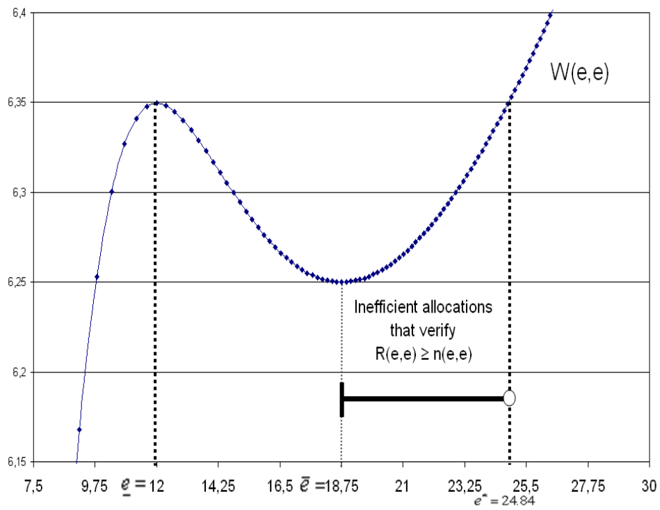
Figure 3: Example 3. Numerical example where the PKD criterium fails to identify dynamically efficient allocations. Above the R(e,e)/n(e,e) function. Below the indirect utility function for the stationary allocations. (Parameters \delta = 1/3 , \gamma = 1/3 , A = 1 , B = 3 , \rho = 1/2 , and \beta = 1 .)
